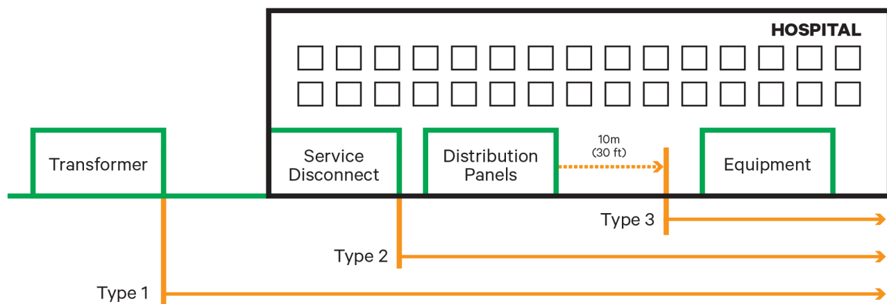
Figure 4: UL 1449 SPD Types
