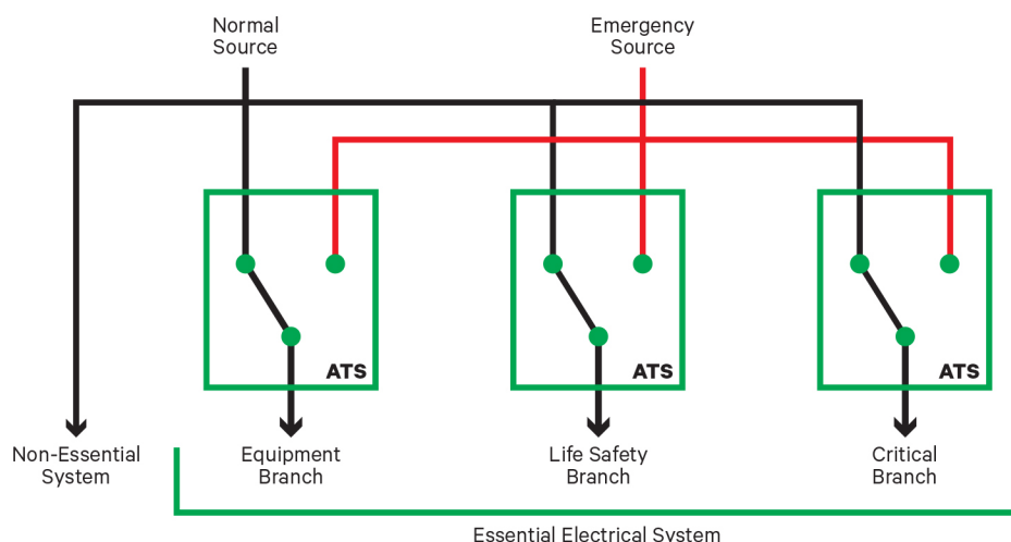
Figure 1: NEC Essential System Configuration
